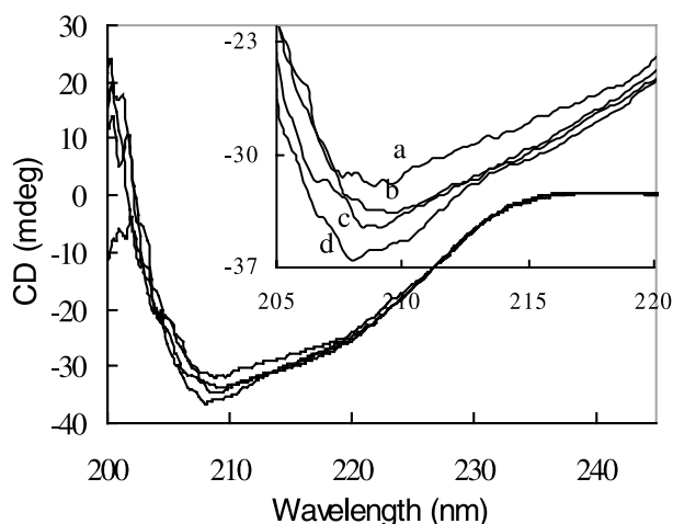
Fig. 1. Effects of salt and Ni 2+ on the BpUreE conformation. Far-UV CD spectra were obtained at 20°C with 5 \mu M BpUreE in 20 mM sodium phosphate buffer (pH 6.5) containing no additive (a), and containing 0.5 M NaCl (b), 10 mM NiCl 2 (c), and both 0.5 M NaCl and 10 mM NiCl 2 (d), respectively. The region from 205 to 220 nm is enlarged in the inset for clarity.
